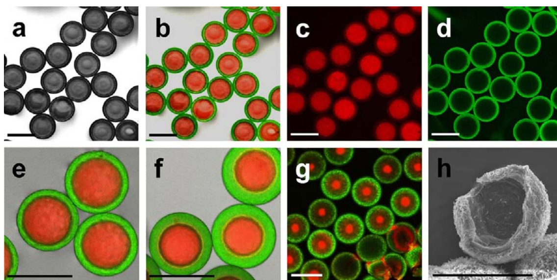
Figure 2. Core-shell particles with the shell consisting of a resolidified lipid and the core formed by an aqueous solution. (a) Light microscopy image depicting the particles in aqueous suspension. (b) Fluorescence detection of the encapsulated drugs: doxorubicin (red) in the core liquid and paclitaxel (green) incorporated within the lipid shell structure. Overlay image. Single component detection for (c) doxorubicin and (d) paclitaxel. The single component images demonstrate that core and shell phases do not show any mixing phase or overlapping signals. (e, f) Different core-shell mass ratios allowing individual encapsulation of drugs within core and shell phase. (g) Solidified particles. The shell structure remains intact upon solidification, and both actives remain effectively encapsulated upon drying. The lower right corner of the figure depicts particles which we crushed on purpose to release the drug for comparison to confirm that the hydrophilic drug remains encapsulated. (h) Electron microscopy image of a cracked lipid shell. The scale bars denote 100 \mu\text{m} .
