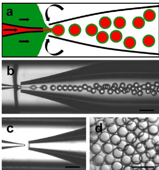
Figure 1. Generation of double emulsion droplets for the formation of core-shell structures in a microcapillary device. (a) Schematic of the device with two adjacently adjusted cylindrical glass capillaries within a square capillary. The device allows the controlled injection of three different fluids. The inner (red) and middle (green) fluids are hydrodynamically focused by the outer fluid (white). (b) Microscopic image of a running device producing core-shell structures. (c) Tapered orifices of the capillaries inside the microfluidic device with a diameter of 20 and 100 \mu\text{m} , respectively (orifices are highlighted by black circles as a guide to the eye). (d) Microscopy image of core-shell particles as the final product. The scale bars denote 200 \mu\text{m} .
